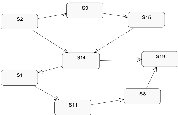
Fig.5 – Dry extreme of SWC.
