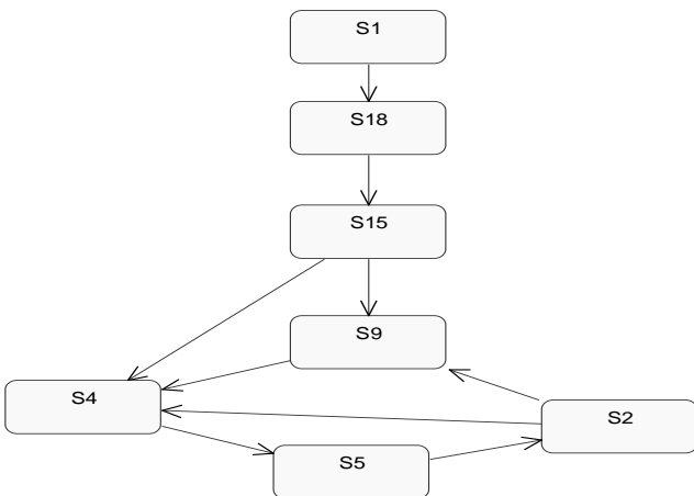
Fig.6 – Stabilizing behavior of the ecosystem.
