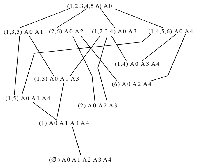
Fig.3 – Hasse diagram constructed from matrix M_G .
