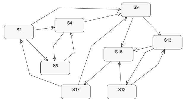
Fig.7 – Standard behavior of ecosystem with SWC.
