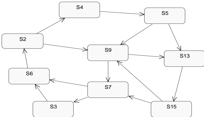
Fig.4 – Moist extreme of SWC.
