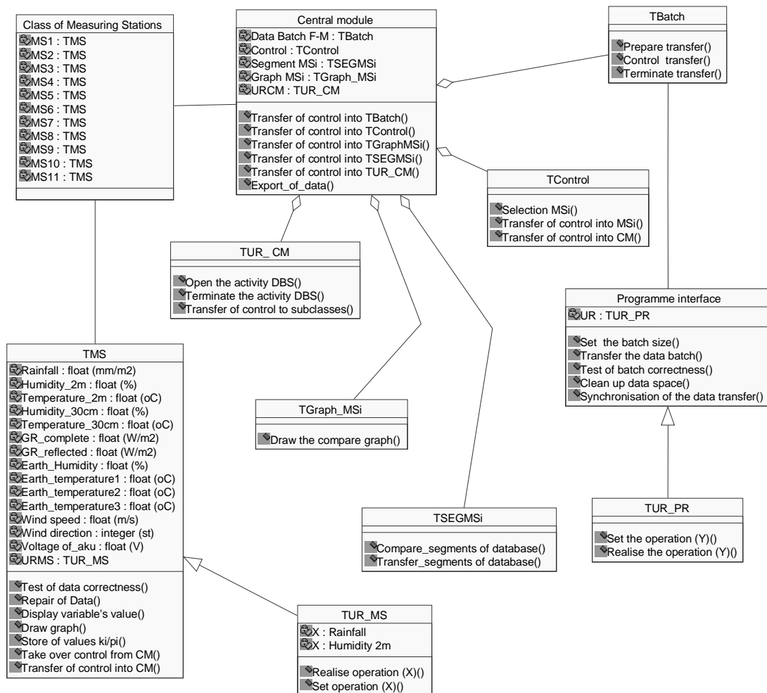
Fig.1 – The schema of database system.
